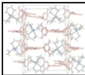
Fig. 2. View along axis a of [\text{Co}(\text{en})_3][\text{B}_5\text{O}_6(\text{OH})_4]_2 \cdot 2 \text{H}_2\text{O} , showing 12 - membered boron rings constructed by O—H···O hydrogen bonds.
